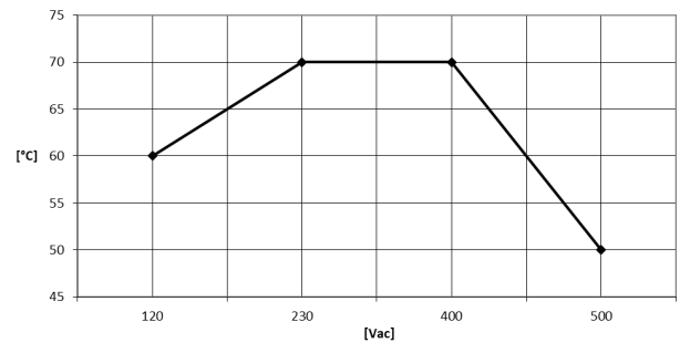
NPSW25-48S - Derating vs Temperature Vout: 48Vdc / Iout: 0.5A
