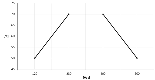
NPSW25-24S - Derating vs Temperature Vout: 24Vdc / Iout: 1.0A
