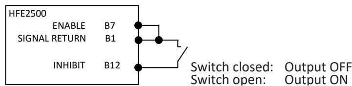
Figure 3–5: Control by INHIBIT
