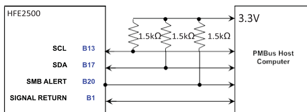
Figure 5–1: PMBus Typical Connection
