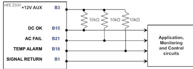
Figure 3-15: Signals
