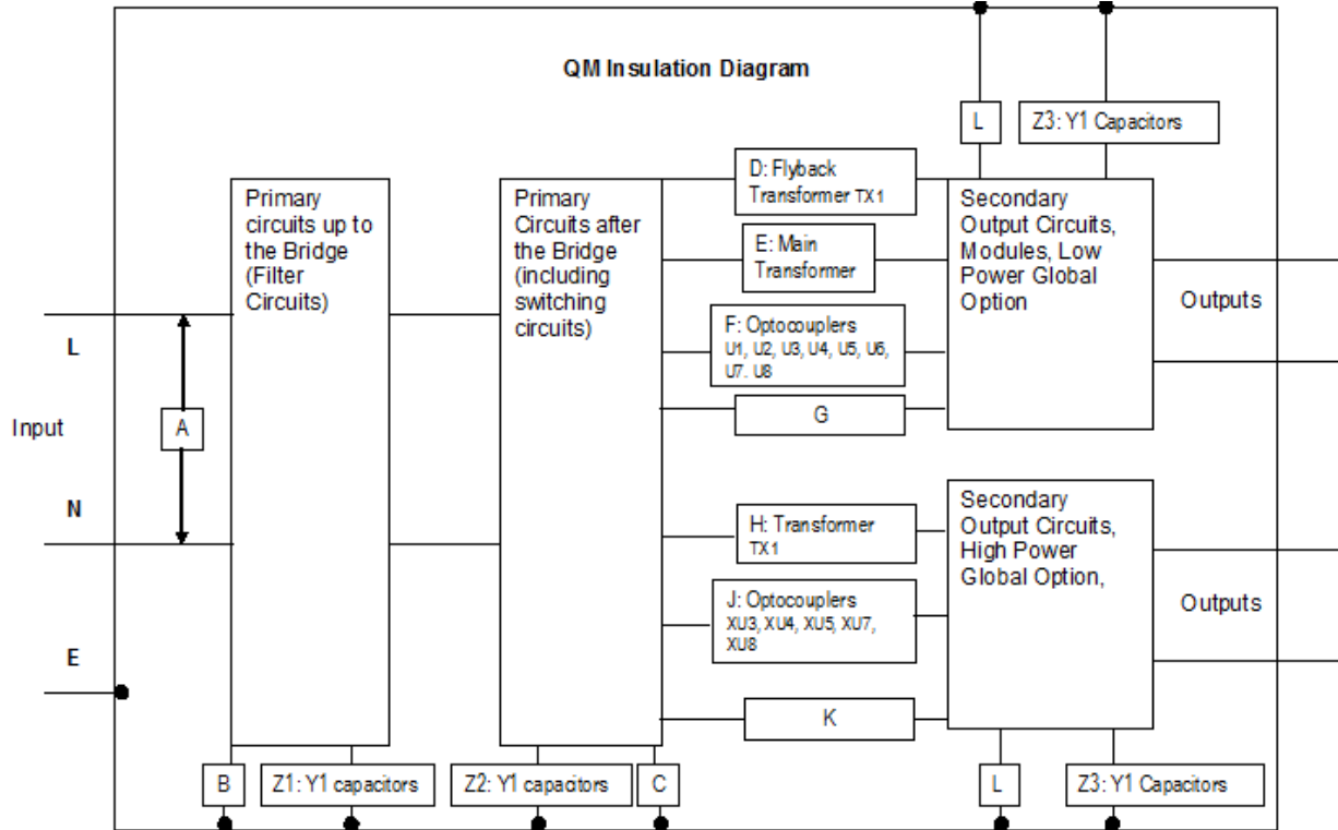
Insulation Diagram - (001) Insulation Diagram
