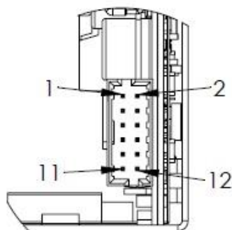
DETAIL L
