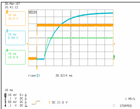
Start-up from Input Voltage Application at Full Load. Ch. 1: Vin Ch. 3: Vo Ch. 4: Io
