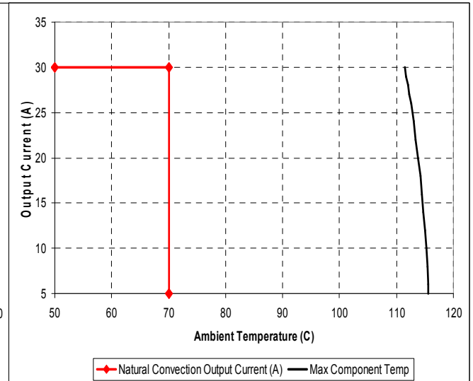
Maximum output current vs. ambient temperature at nominal input voltage for airflow rates natural convection (0.3m/s) and up with airflow from pin 1 to pin 4.
