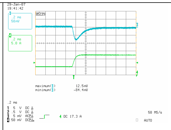
Load Transient Response. Load Step from 50% to 75% of Full Load with di/dt= 0.1A/uS. Ch. 3: Vo Ch. 4: Io
