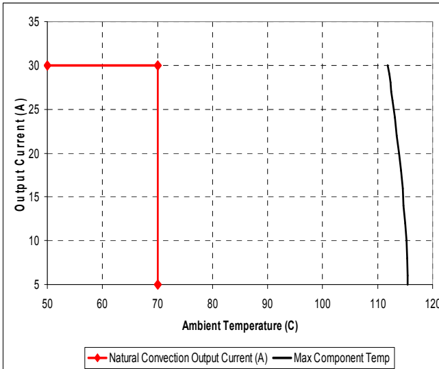
Maximum output current vs. ambient temperature at nominal input voltage for airflow rates natural convection (0.3m/s) and up with airflow from pin 4 to 1.
