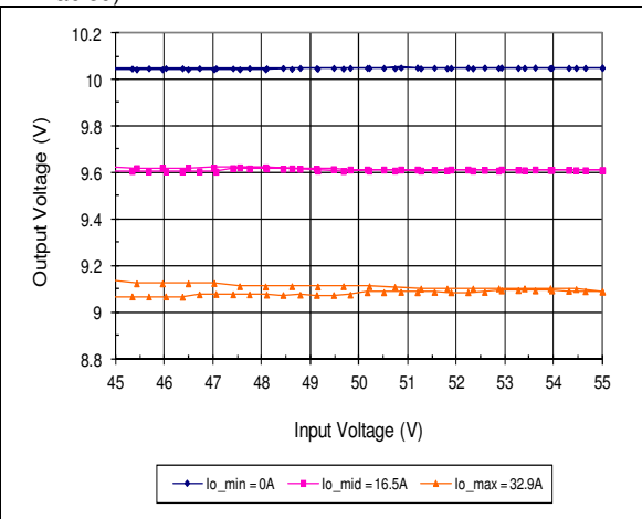
Typical Output Voltage vs. Vin at Ta=55C (Droop Feature Enabled)
