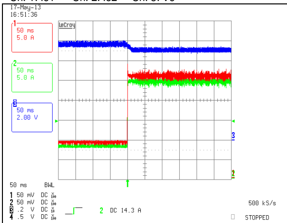
Load Transient Response. Load Step: 16.5A to 49.5A, 0.1A/us slew rate. Ch. 1: lo1 Ch. 2: lo2 Ch. 3: Vo
