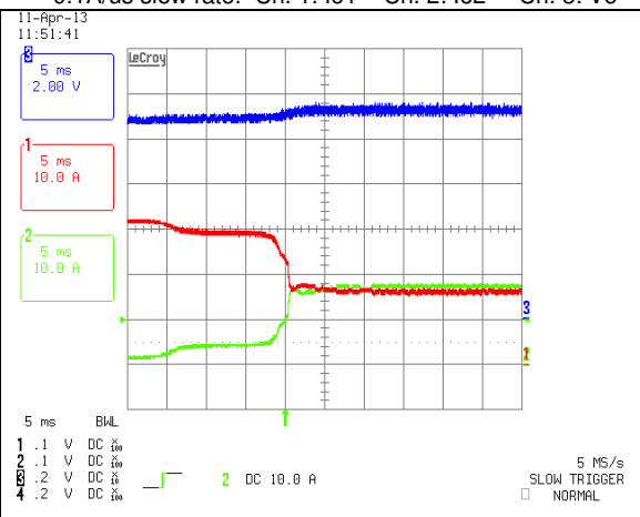
Start-up with back-biasing: Vin=50V, Io=33A Ch. 1: lo1 Ch. 2: lo2 Ch. 3: Vo
