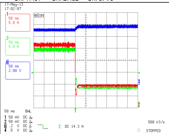
Load Transient Response. Load Step: 49.5A to 16.5A, 0.1A/us slew rate. Ch. 1: lo1 Ch. 2: lo2 Ch. 3: Vo
