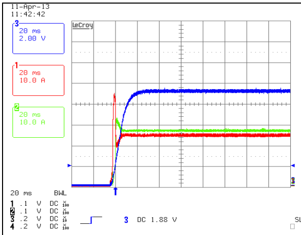
Start-up from ON/OFF Switch: Vin=50V, Io=50A Ch. 1: lo1 Ch. 2: lo2 Ch. 3: Vo
