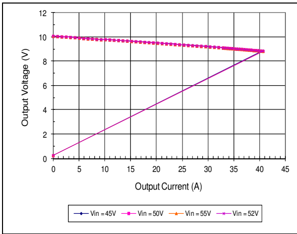
Load Current Limit Characteristics vs. Vin (Droop Feature Enabled)
