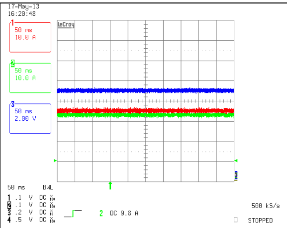
Steady State Load Share: Vin=50V, Io=66A Ch. 1: lo1 Ch. 2: lo2 Ch. 3: Vo
