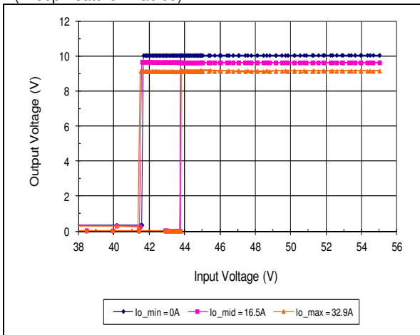
Typical Output Voltage vs. Low Voltage Input Turn-on and Turn-off (Droop Feature Enabled)
