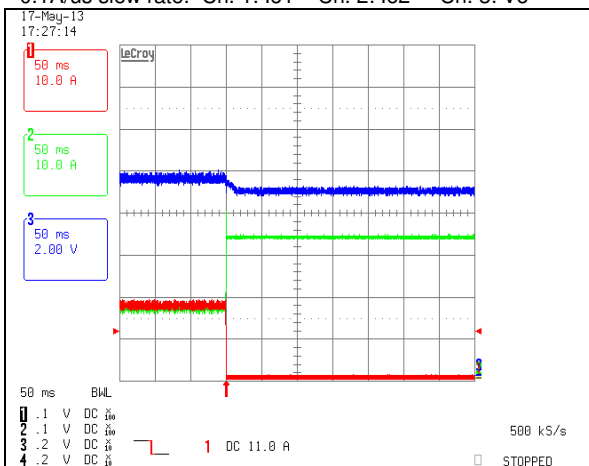
Shut-down when running Io=33A (100% Load) Ch. 1: lo1 Ch. 2: lo2 Ch. 3: Vo
