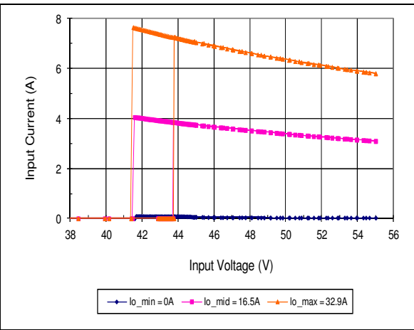
Typical Input Current vs. Vin (Droop Feature Enabled)
