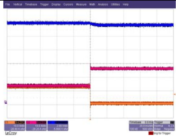
Shut-down when running I o =50A load (200% Load) Ch. 1: I o1 Ch. 2: I o2 Ch. 3: V o
