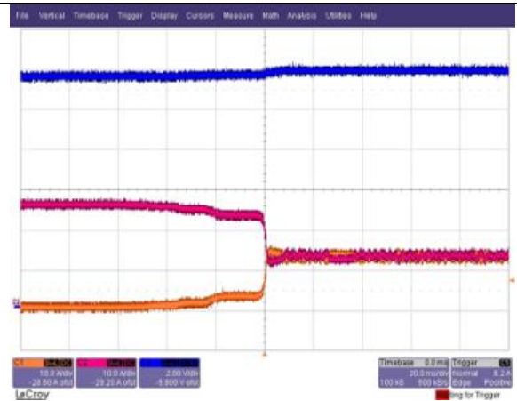
Start-up with back-biasing: V in =48V, I o =25A Ch. 1: I o1 Ch. 2: I o2 Ch. 3: V o
