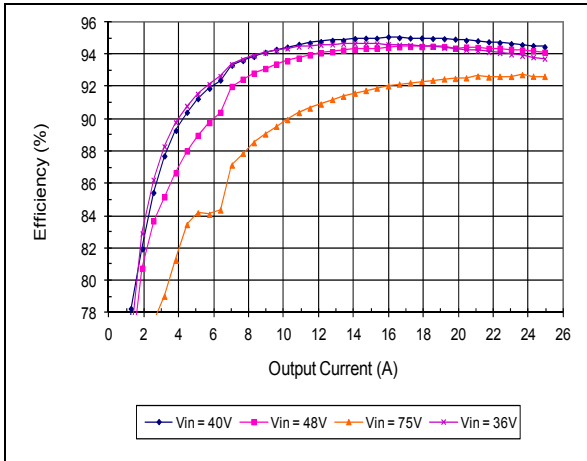
Efficiency at various lines and loads (test in socket, 25C)
