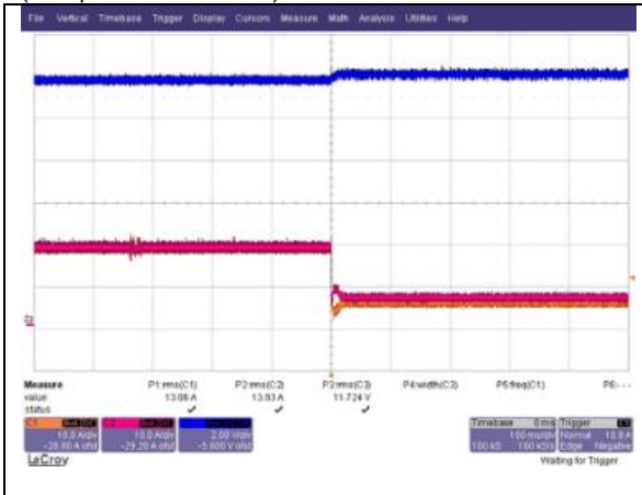
Load Transient Response. 37A to 12A (74% to 24%), 0.1A/us slew rate. Ch. 1: I o1 Ch. 2: I o2 Ch. 3: V o
