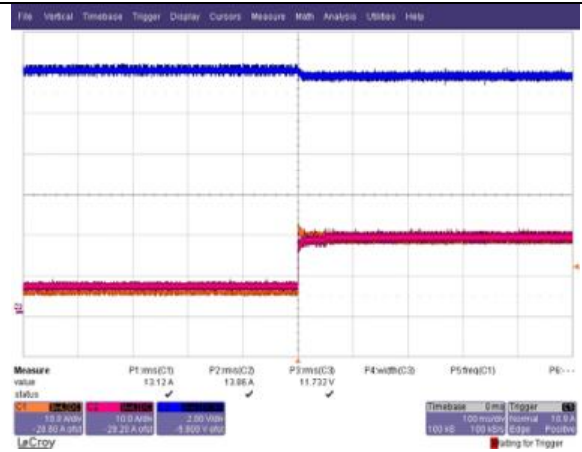
Load Transient Response. 12A to 37A (24% to 74%), 0.1A/us slew rate. Ch. 1: I o1 Ch. 2: I o2 Ch. 3: V o
