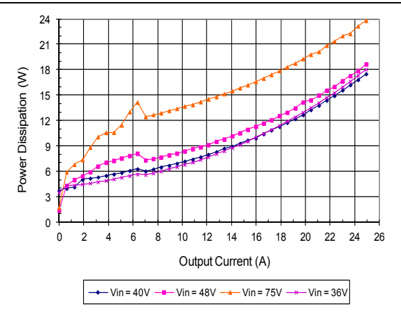
Power Dissipation at various lines and loads (test in socket, 25C)
