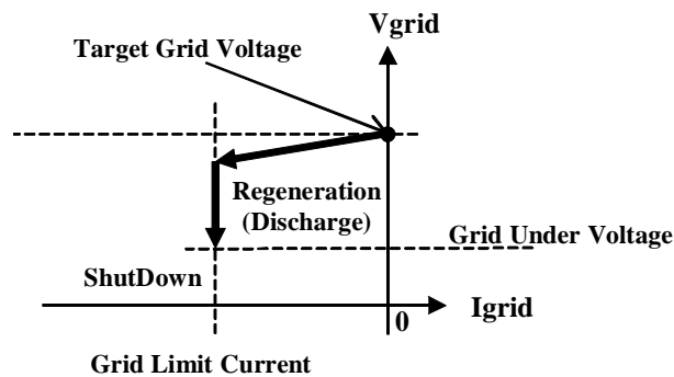
Operating Characteristic
