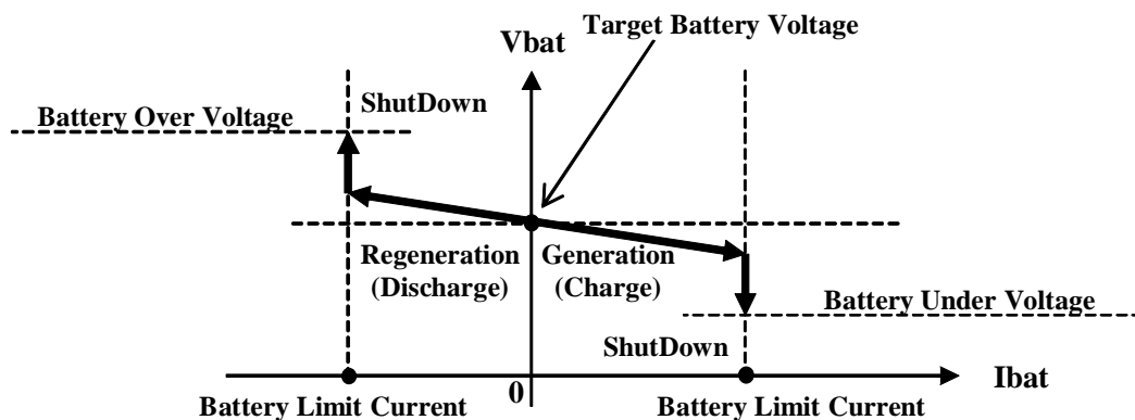
Operating Characteristic
