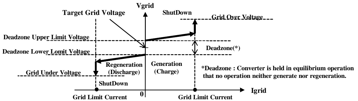
Operating Characteristic
