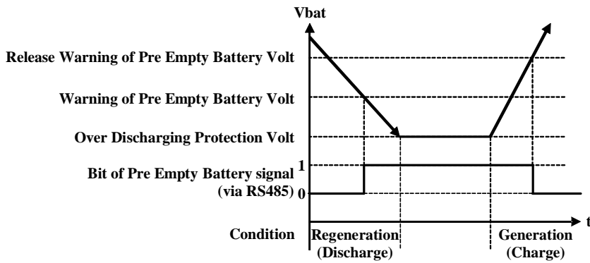
Battery Over Discharging Protection Timing Chart
