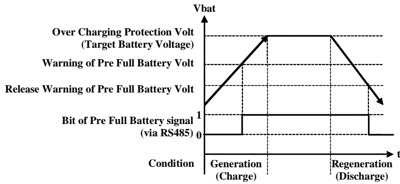
Battery Over Charging Protection Timing Chart
