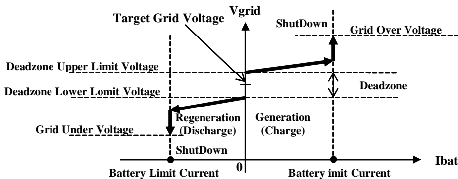
Operating Characteristic
