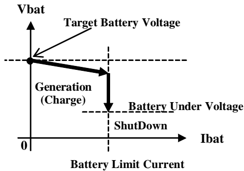
Operating Characteristic
