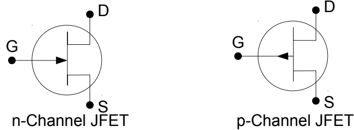
Drawing 17: Schematic Symbols for J-FETs
