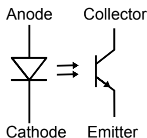
Drawing 21: Schematic Symbol for an Opto-Coupler
