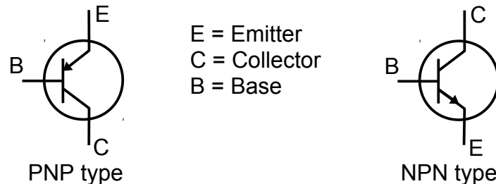
Drawing 2: Schematic Symbols for BJT's
