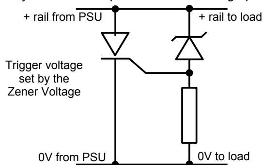
Drawing 5: Overvoltage Crowbar Circuit
