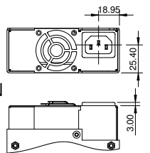
FAN+IEC OPTION
