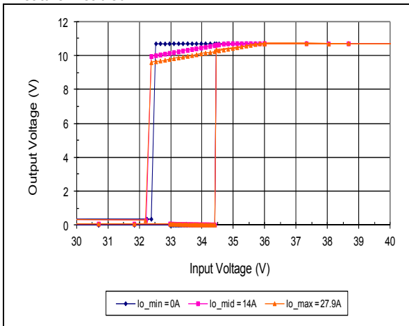
Typical Output Voltage vs. Low Voltage Input Turn-on and Turn-off
