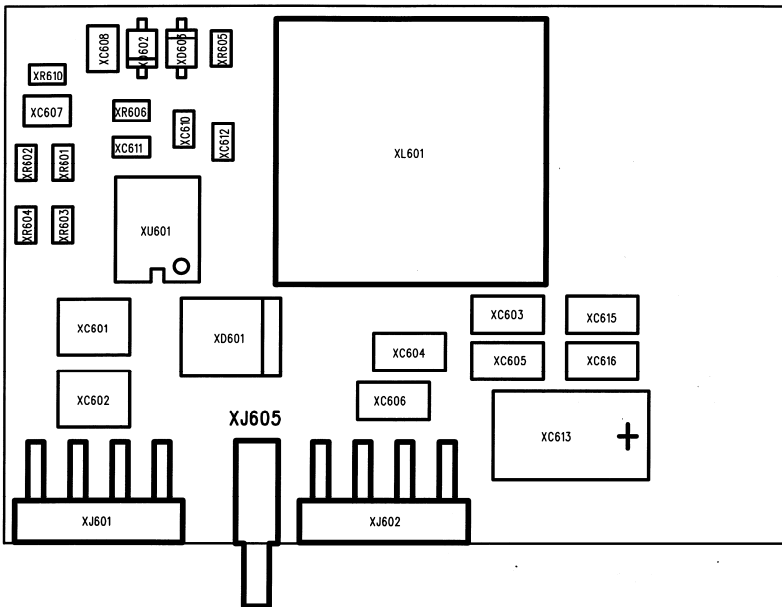
SMA 4 board (Ch4)
