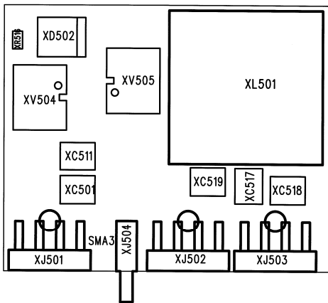
SMA 3 board (Ch3, O/Ps TH and FH)
