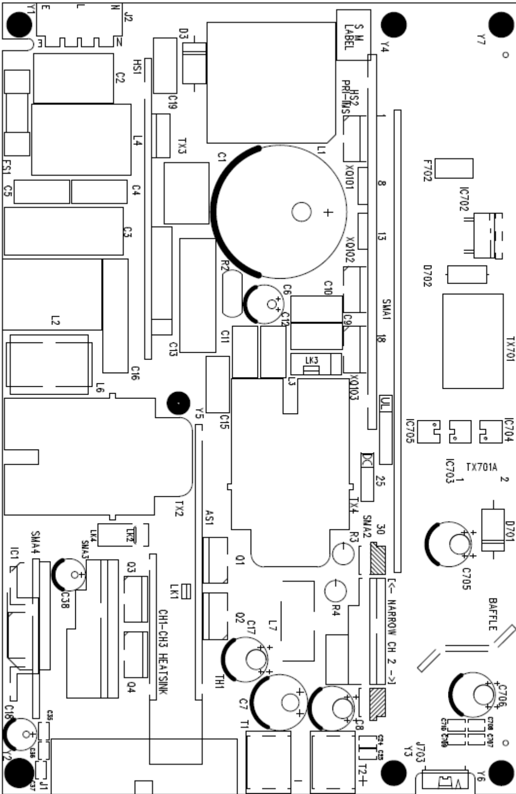
Base board (Wide)
