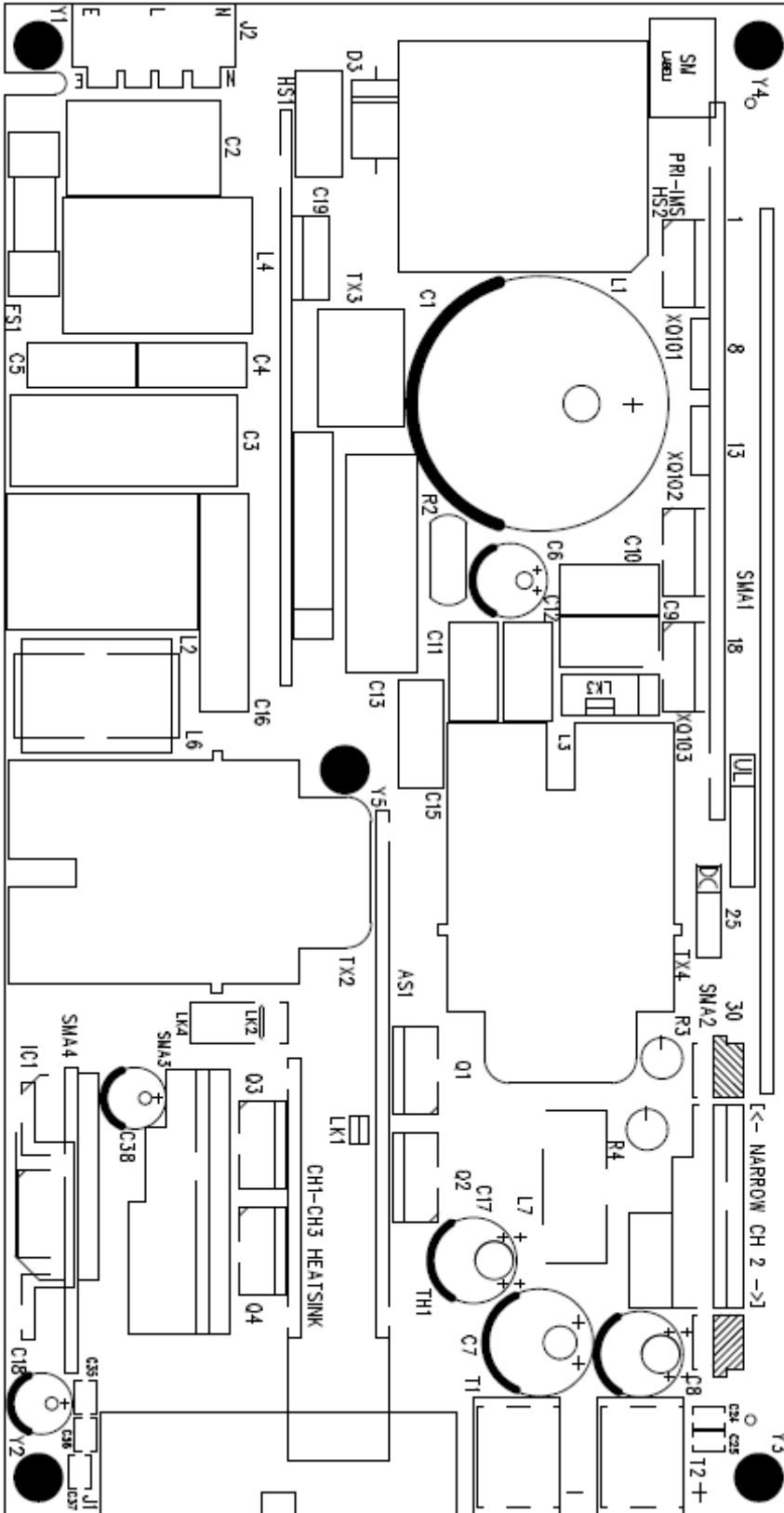
Base board (Narrow)
