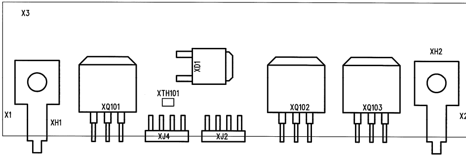
Primary IMS board
