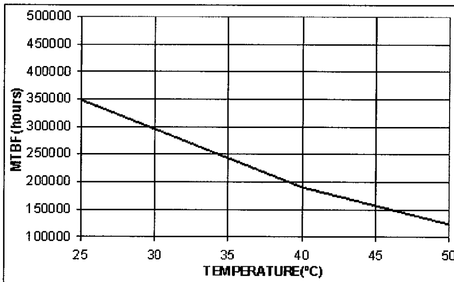
TEMPERATURE CURVE
