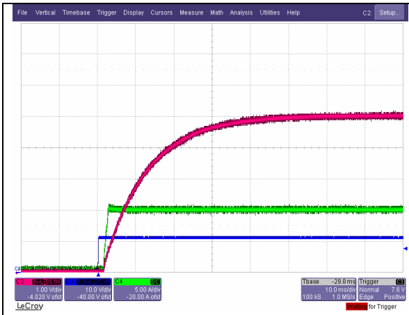
Start-up from on/off Switch at 48V input and Full Load. Ch. 2: Vo Ch. 3: ON/OFF Ch. 4: Io
